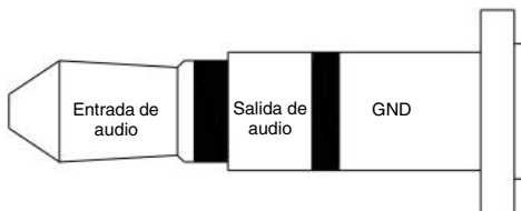
Figura: Miniconector de audio TRS.
